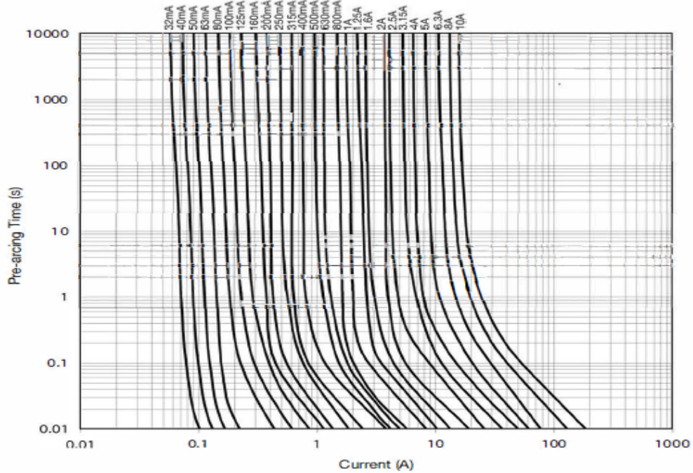
Nominal Time-Current Characteristics
